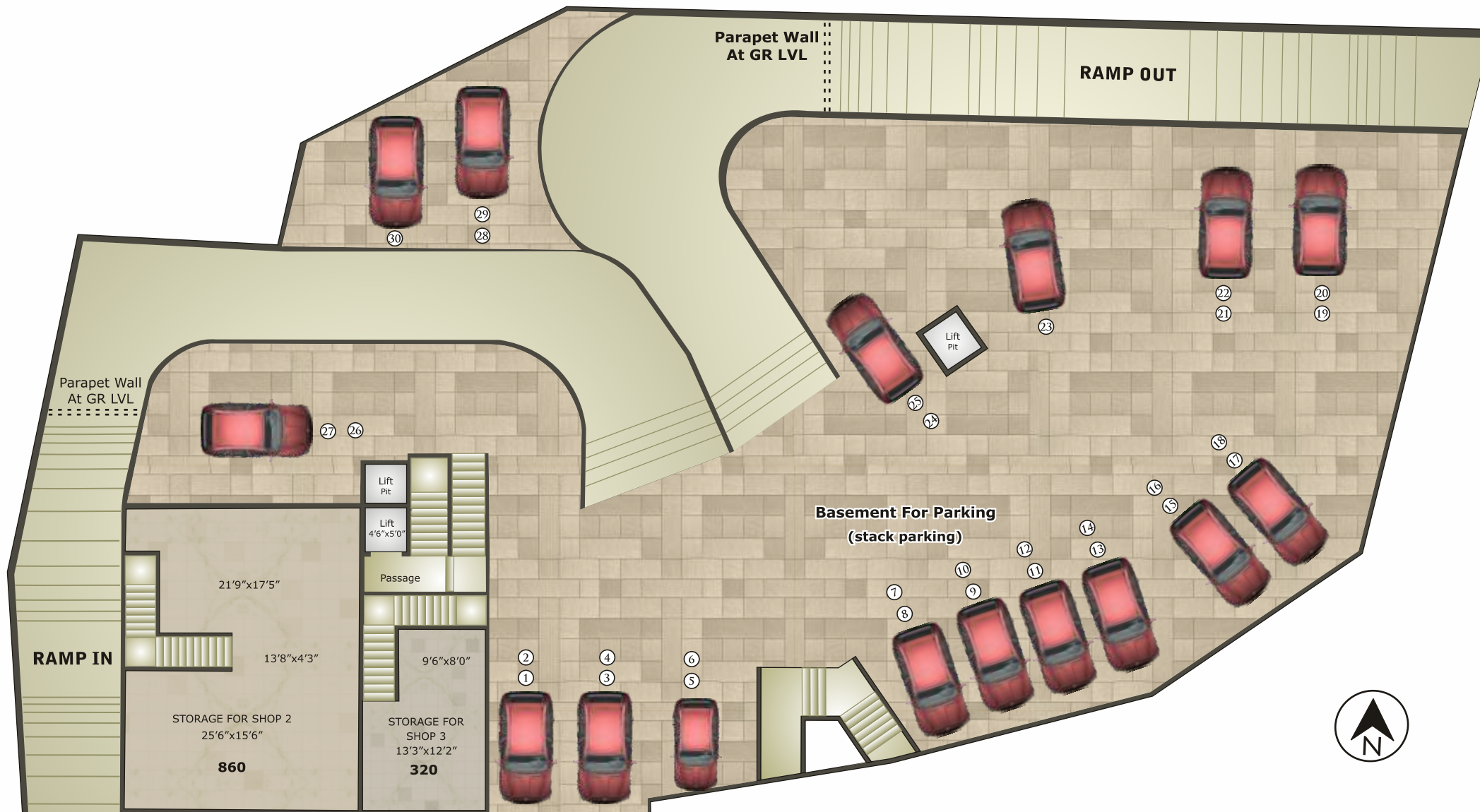
Basement Plan
